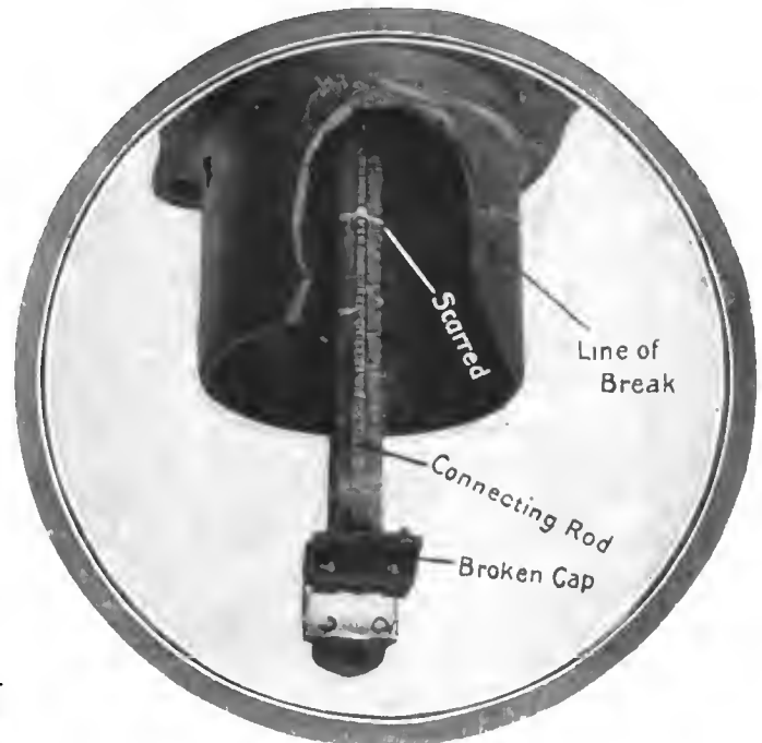
Fig. 2—Illustrating a broken cylinder which was caused by the failure of one of the connecting rod bolts. The following revolution of the crankshaft drove the connecting rod through the cylinder
